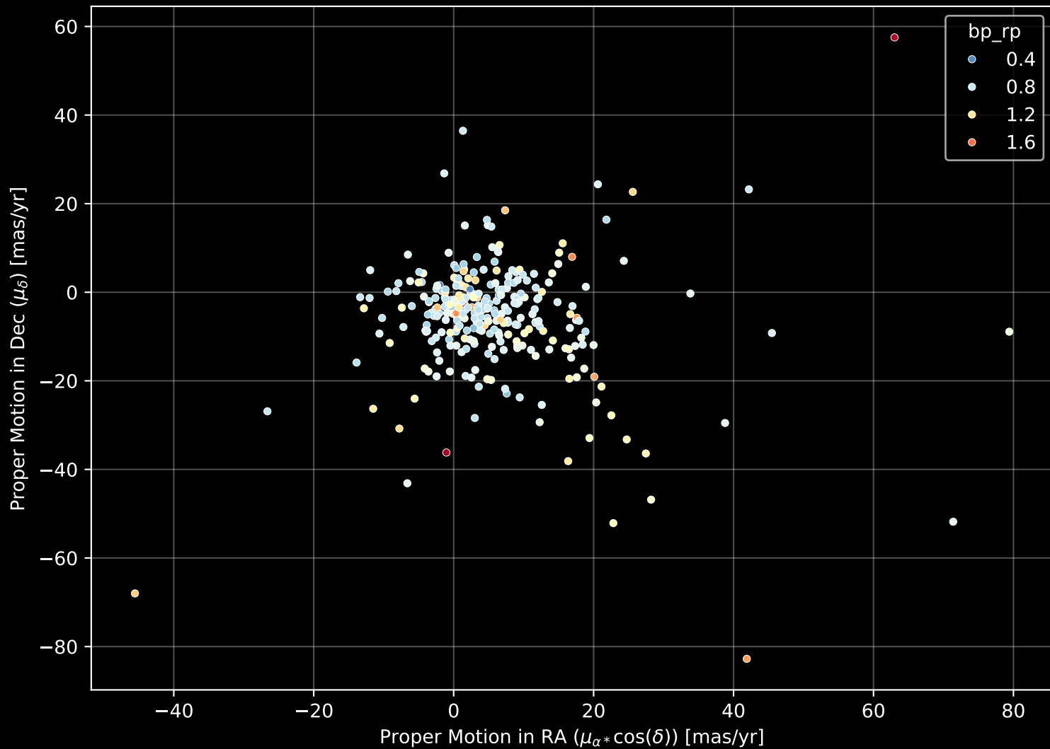
GALAH DR4 Field: [999] Proper Motion Diagram (n= 297)
