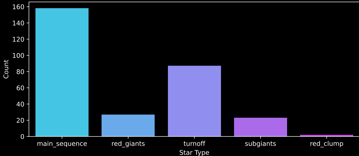
GALAH DR4 Field: [999] Count plot of Star Type
