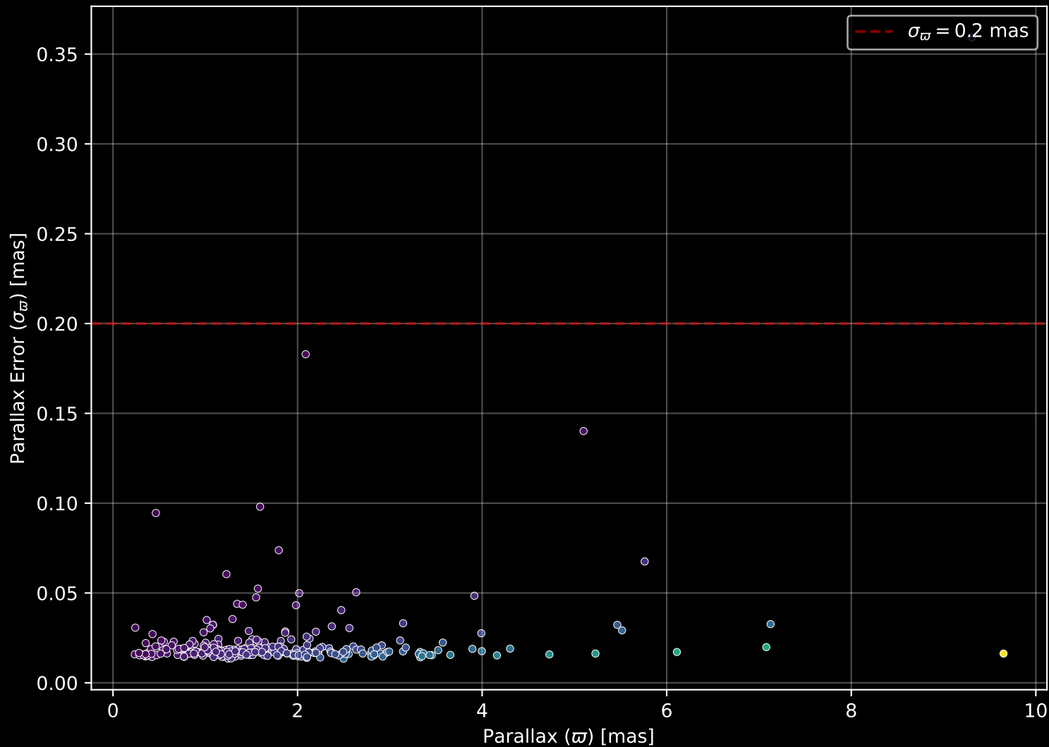
GALAH DR4 Field: [999] Parallax Quality (n= 297)
