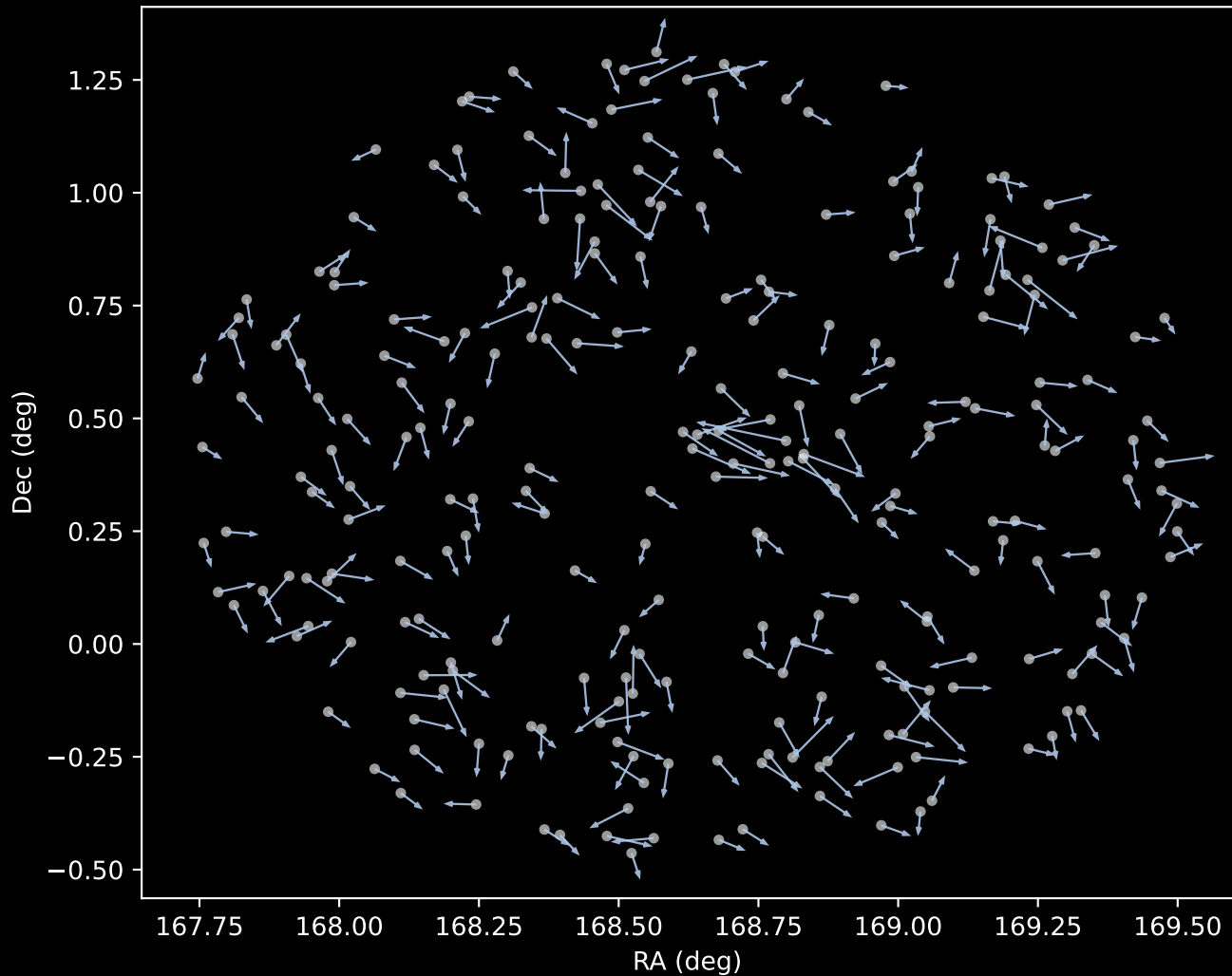
GALAH DR4 Cluster 1 Proper Motion Vectors (n=254)
