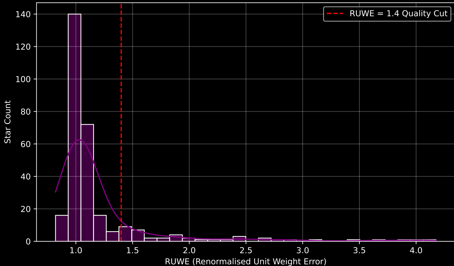
GALAH DR4 Field [999] RUWE Distribution (n= 292)
